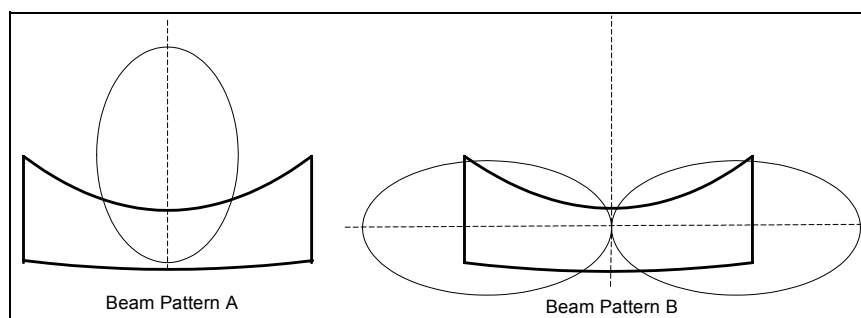
Figure 5 EUM3005 Switched-beam Diversity Antenna — Beam Patterns
